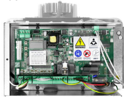
Control unit with built-in inverter, LCD display and encoder
