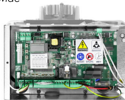
Control unit with built-in inverter, LCD display and virtual encoder
