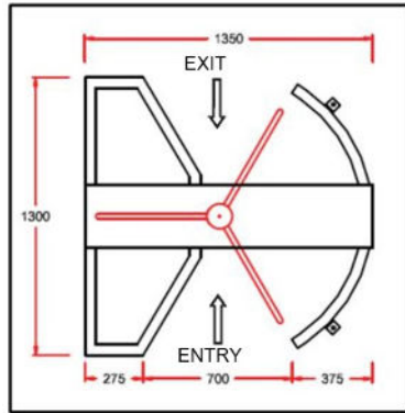
STANDARD TURNSTILE
