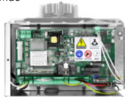
Control unit with built-in inverter, LCD display and virtual encoder
