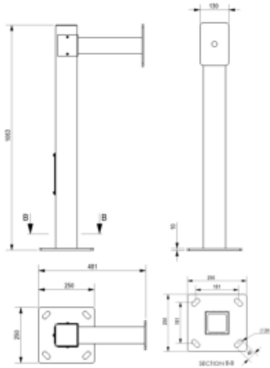
Single card reader assembly no box
