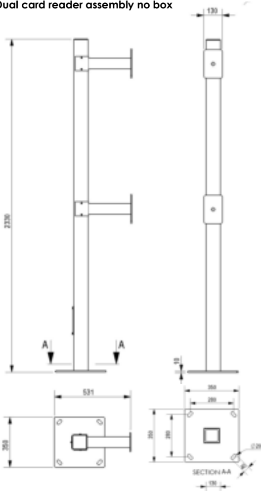
Dual card reader assembly no box
