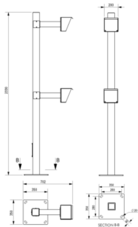
Dual card reader assembly with box
